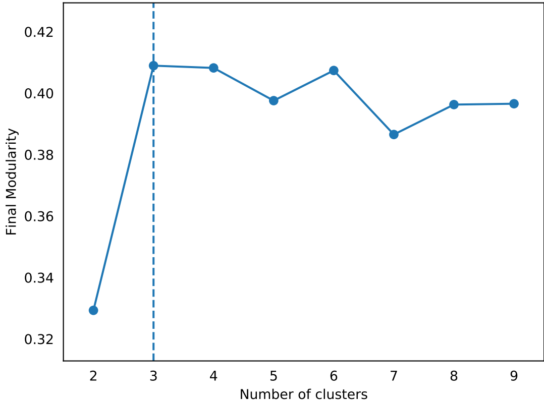
Max. modularity for 3 clusters (0.4089)
