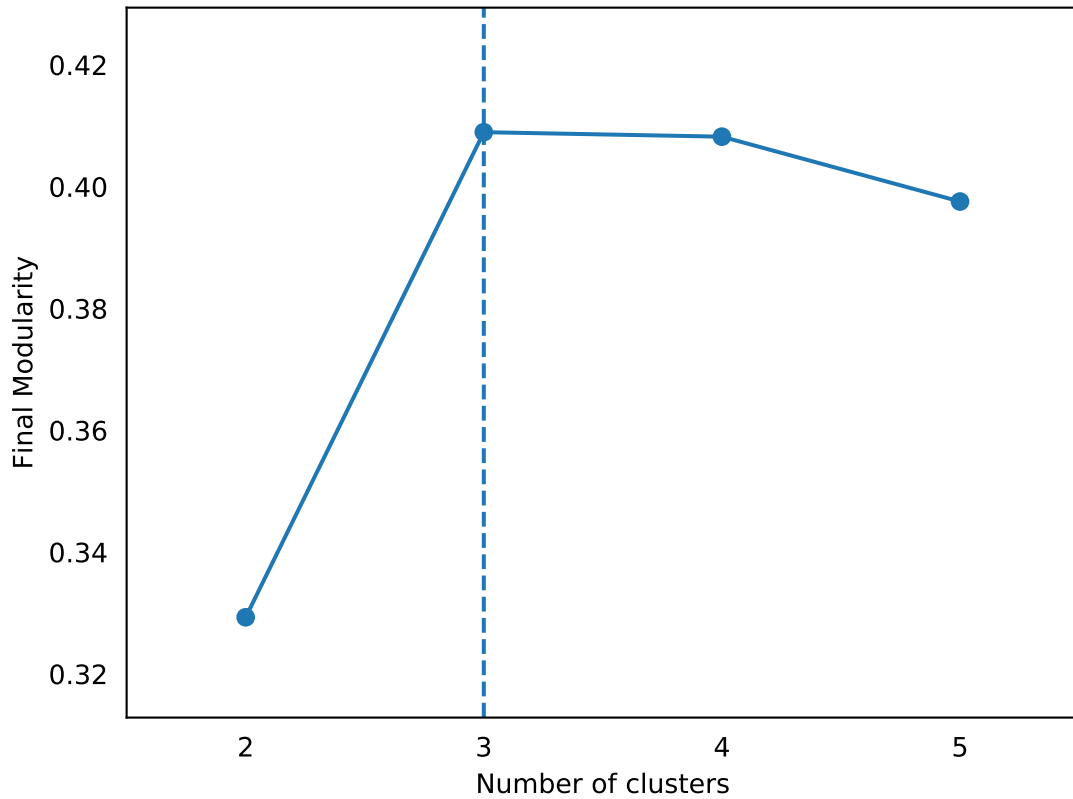
Max. modularity for 3 clusters (0.4089)
